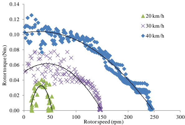
Fig. 9: Rotor speed as a function of torque for the 16-blade rotor without a cowling.
