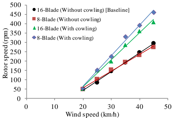
Fig. 10: Maximum rotor speed vs. wind speeds.
