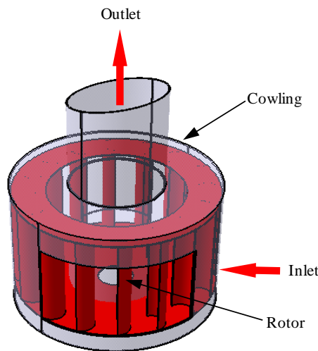
Fig. 5: Wind turbine rotor including the cowling assembled together.
