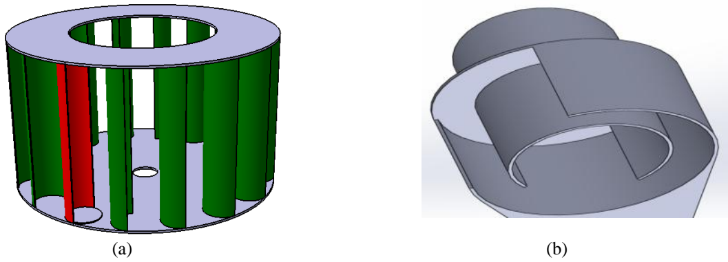
Fig. 4: (a) A 3D model of the 16-bladed turbine rotor and (b) the cowling device.
