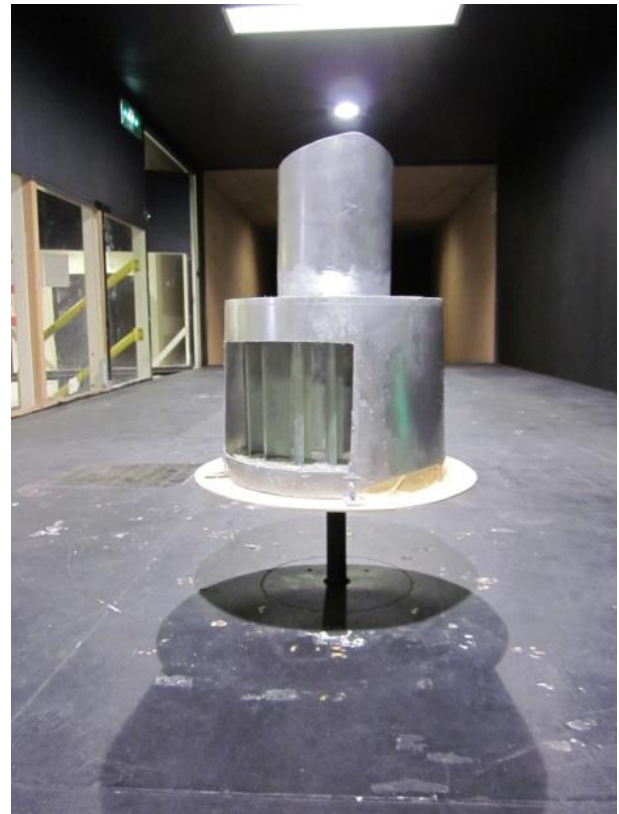
Fig. 8: Experimental setup inside the RMIT Industrial Wind Tunnel.
