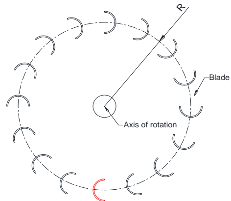
Fig. 2: Top view of 16-bladed wind turbine rotor.
