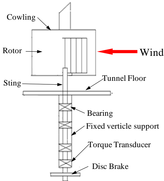
Fig. 7: Schematic of the experimental setup.
