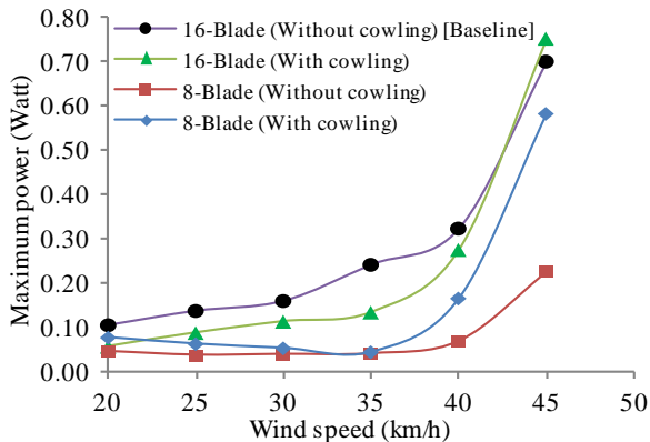
Fig. 11: Maximum power as a function of wind speeds.
