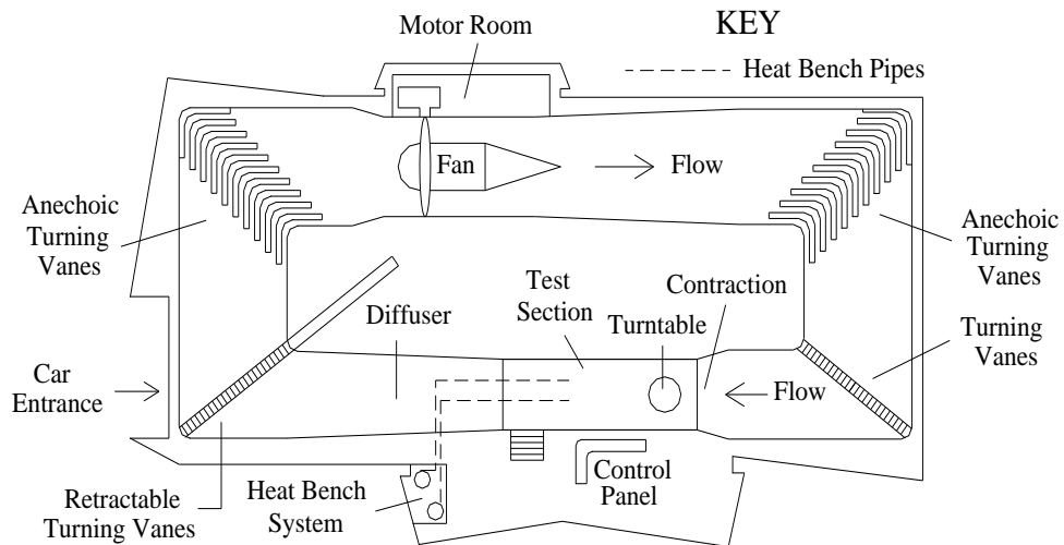
Fig. 6: A plan view of RMIT Industrial Wind Tunnel.
